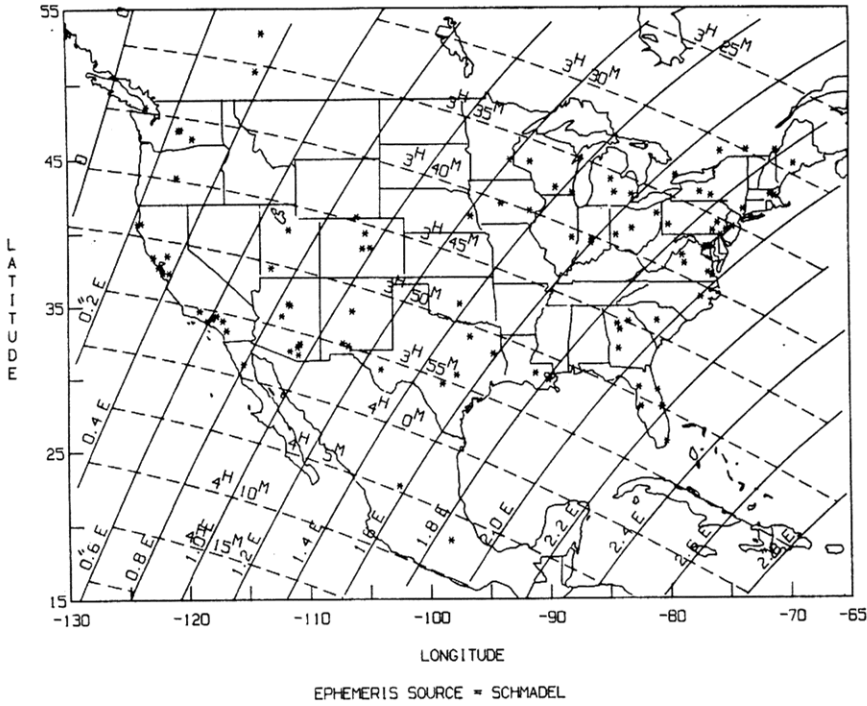
1987 2 9 (10) HYGIEA DIAMETER 443 KM = 0".21
