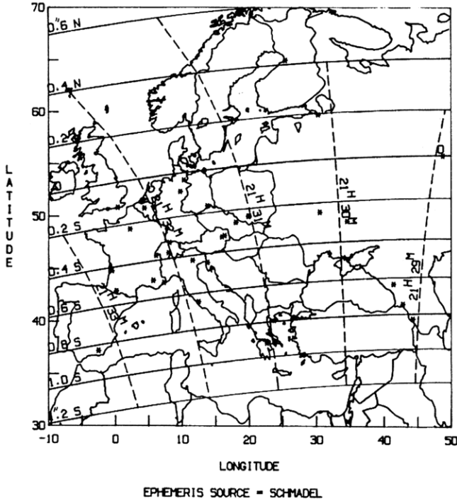
1987 1 27 (704) INTERAMNIA DIAMETER 338 KM = 0".21
